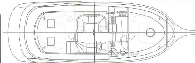
MAIN DECK
