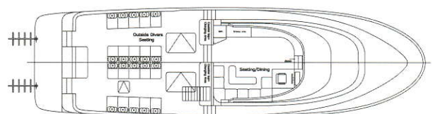
MAIN DECK
