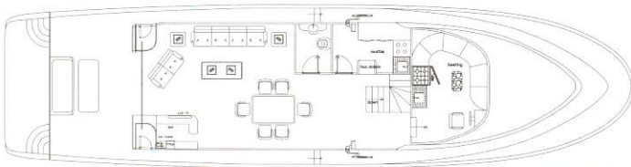
MAIN DECK
