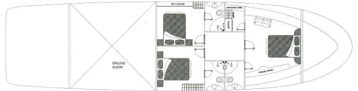
INTERIOR DECK
