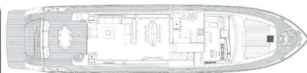
MAIN DECK
