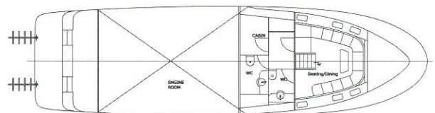
LOWER DECK
